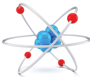
This is an atom.
