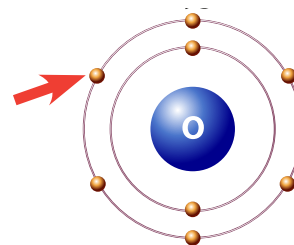
This is an electron.
