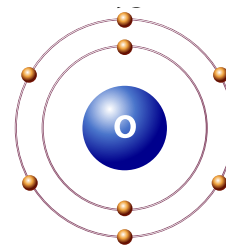
This is an atom.
